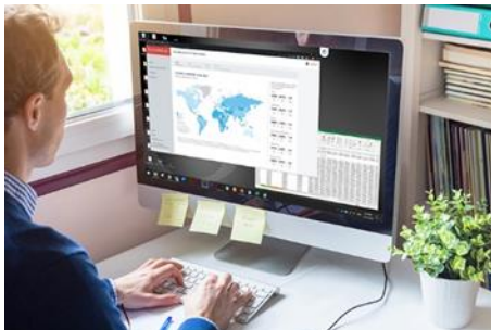
Country-level data
